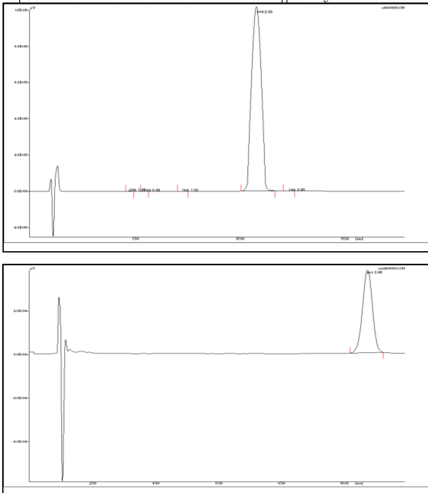
Figure No.7: Ibuprofen tablets I4 solution (1) and (2)
