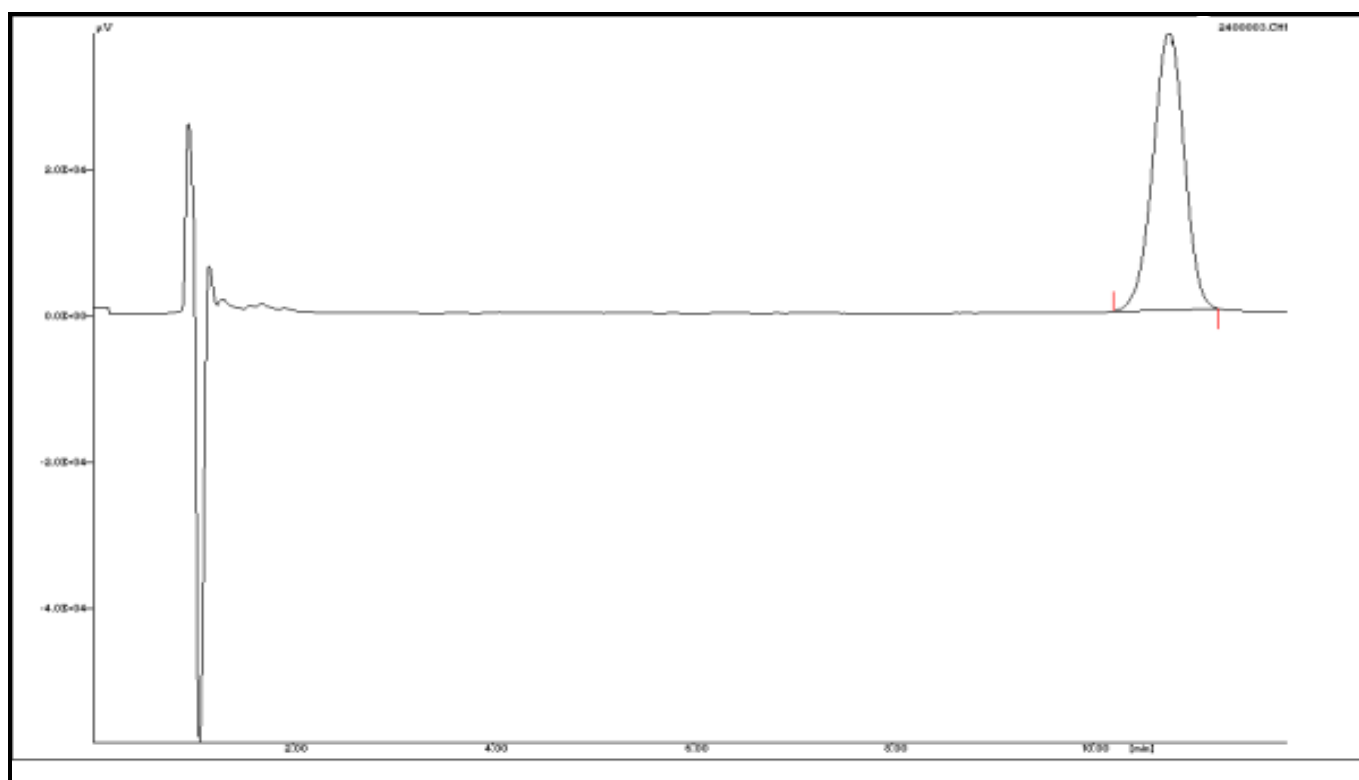
Figure No.6: Ibuprofen tablets I3 solution (1) and (2)
