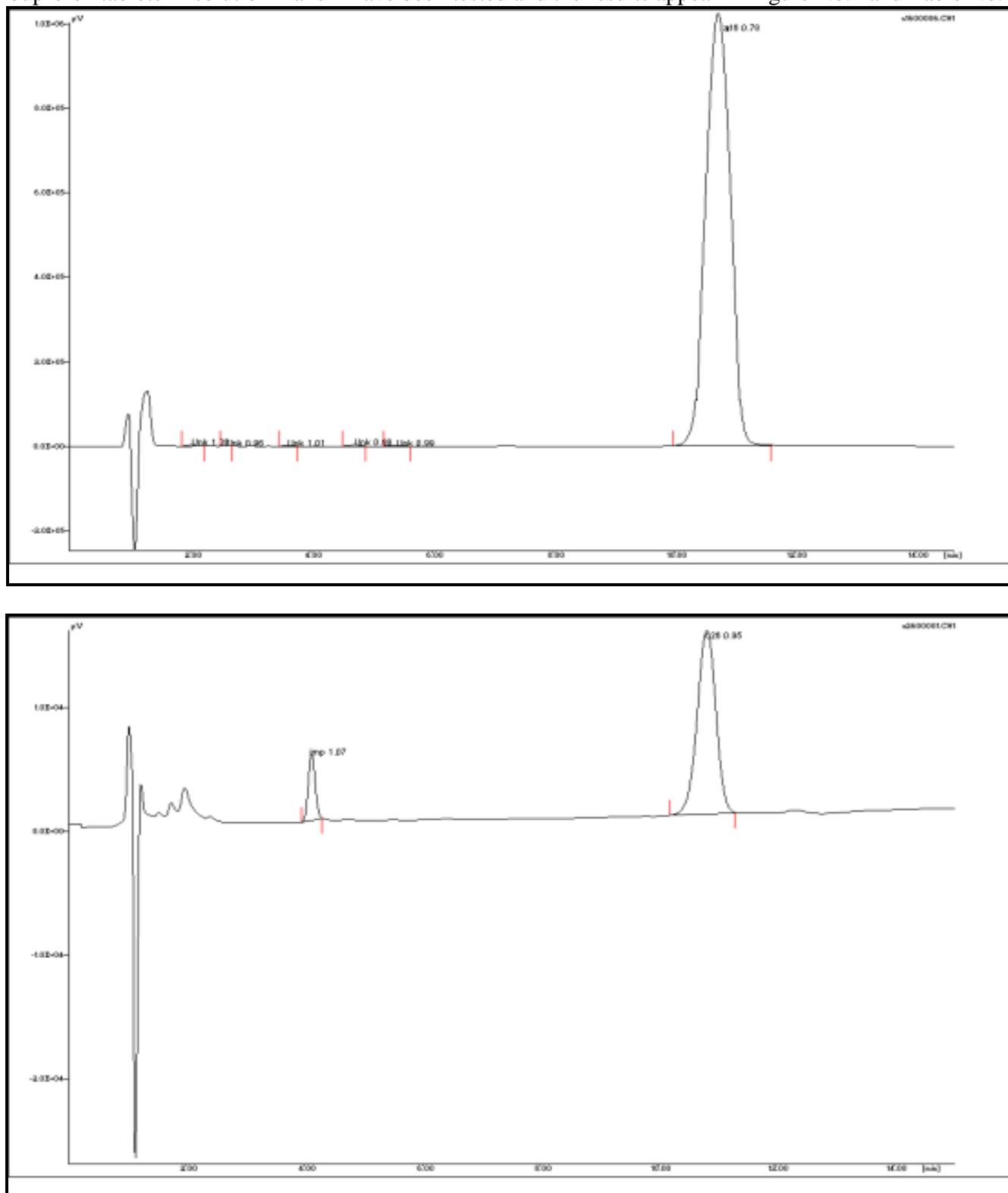
Figure No.4: Ibuprofen tablets II solution (1) and (2)
