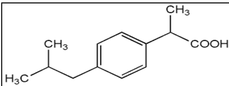
Figure No.1: Chemical structure of Ibuprofen
