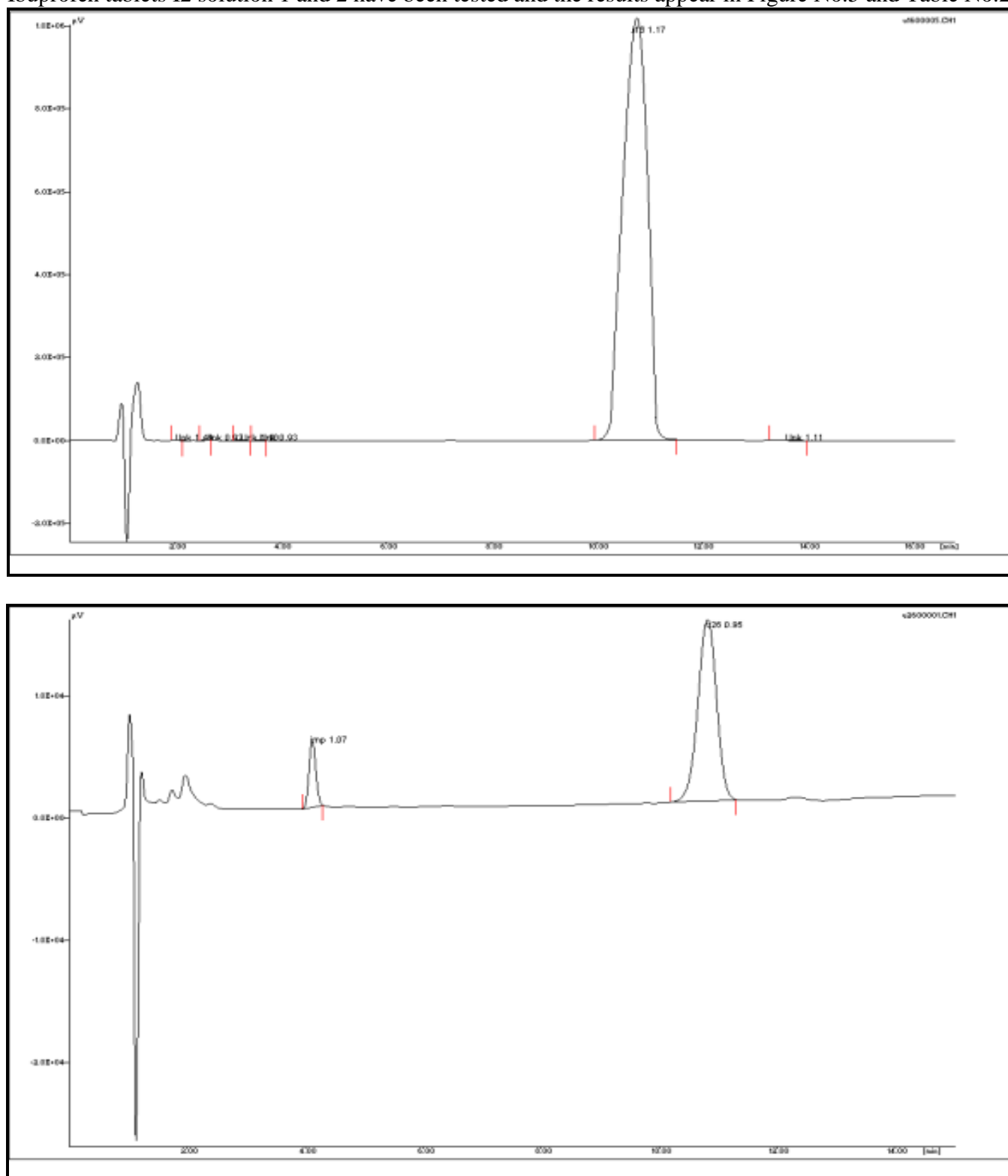
Figure No.5: Ibuprofen tablets I2 solution (1) and (2)
