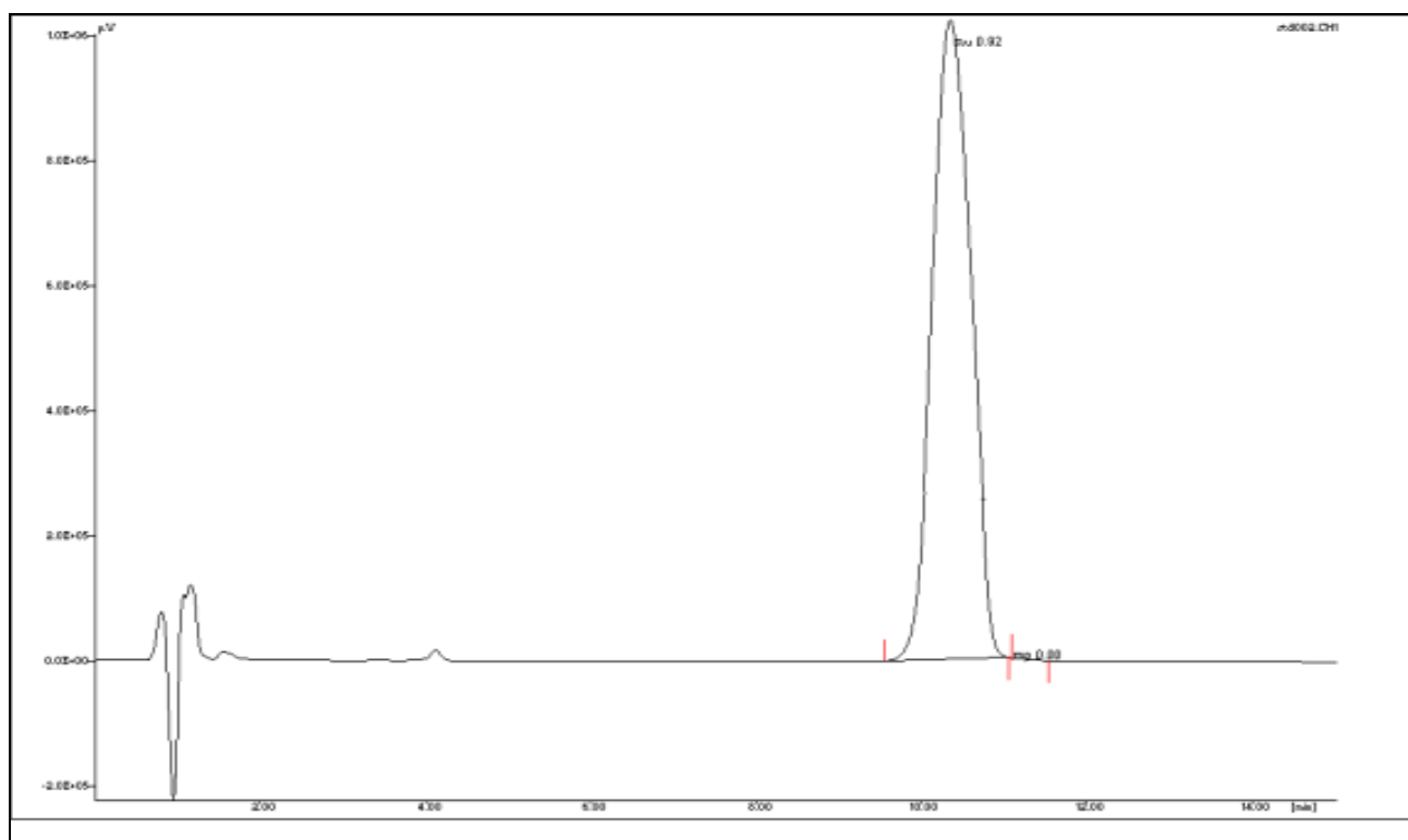
Figure No.3: Standard solution injection for SST
