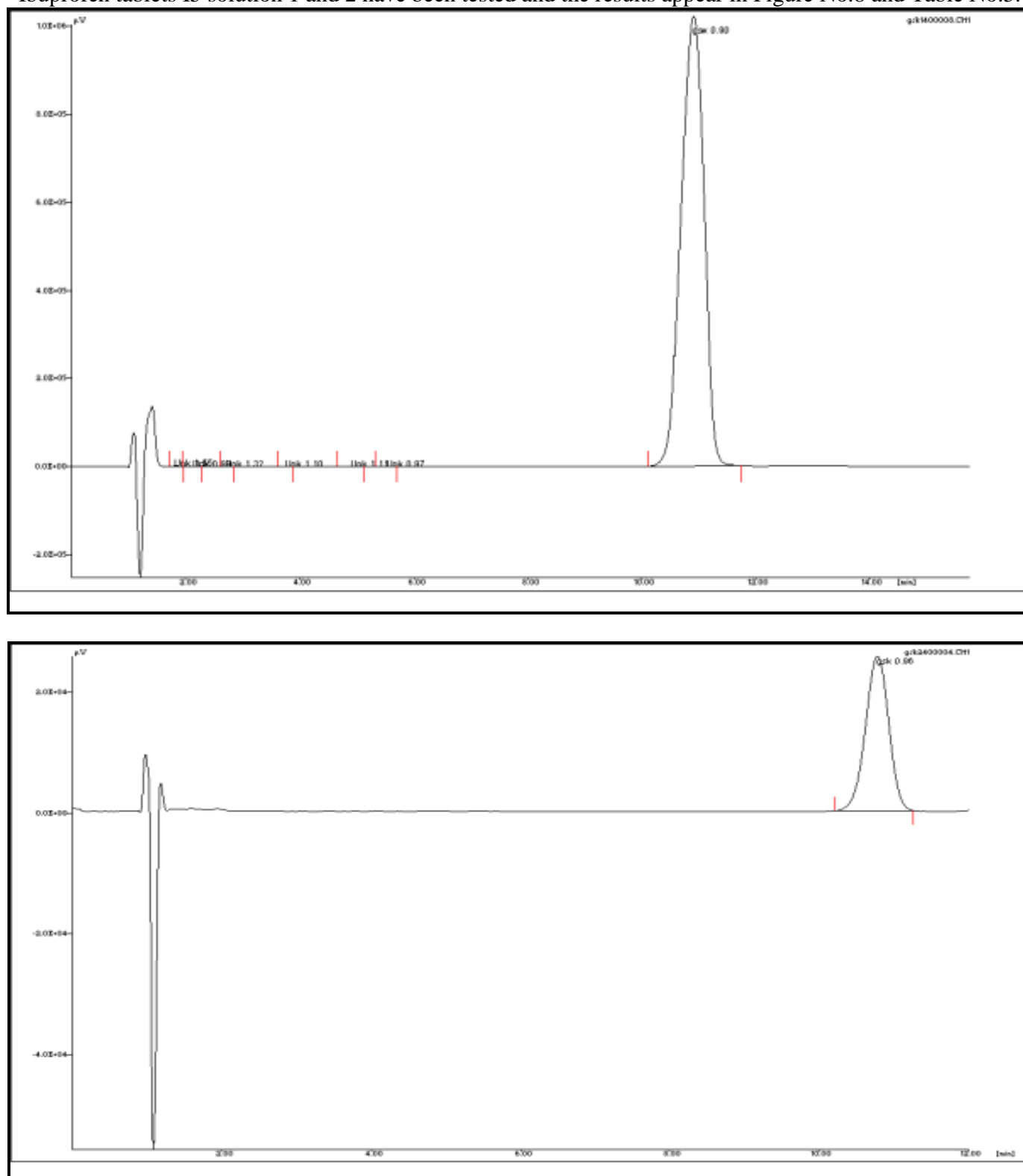
Figure No.8: Ibuprofen tablets I5 solution (1) and (2)
