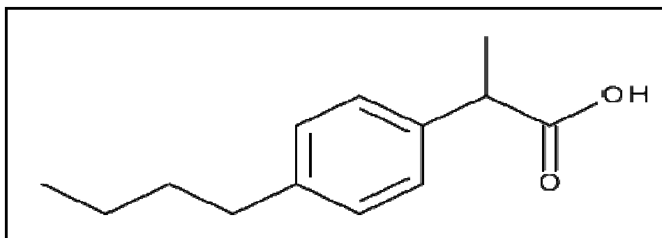
Figure No.2: Chemical structure of Ibuprofen impurity B
