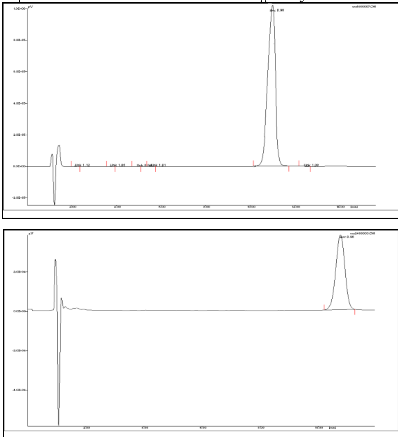
Figure No.9: Ibuprofen tablets I6 solution (1) and (2)
